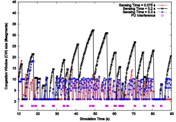
Figure 4. Sensing Cycle Analysis: CW size over Time.
