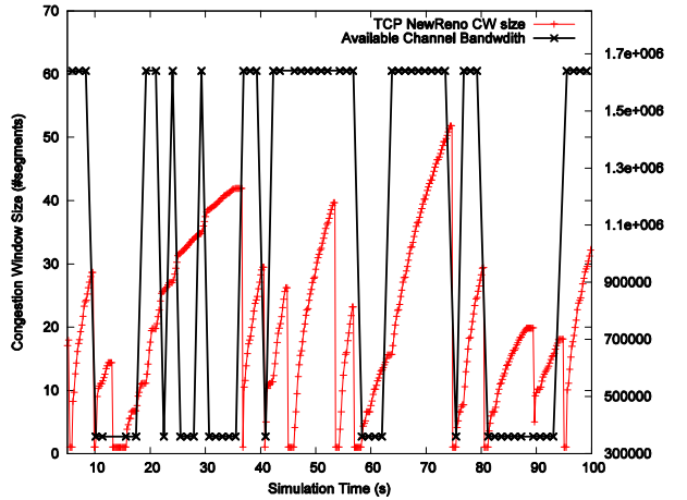
Figure 8. Channel Heterogeneity Analysis: CW size vs Available Bandwidth.
