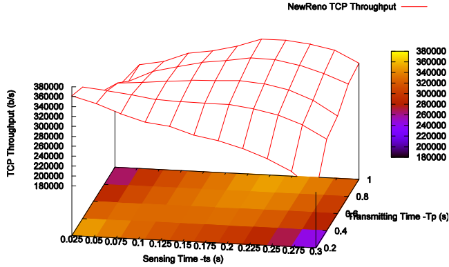
Figure 2. Sensing Cycle Analysis: NewReno TCP Throughput, variable transmitting and sensing time intervals.
