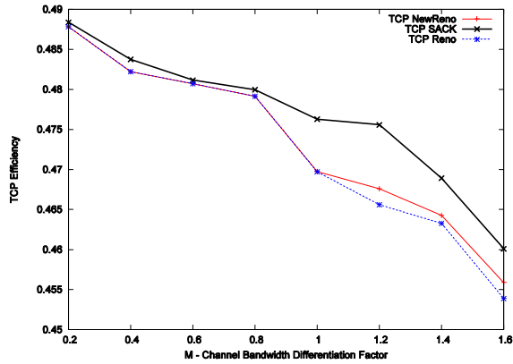
Figure 7. Channel Heterogeneity Analysis: TCP Efficiency.
