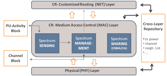
Figure 1. NS-2 Revised Architecture Block.
