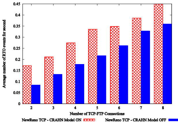
Figure 10. Multi-Hop Topology: Avg. RTO events for seconds.
