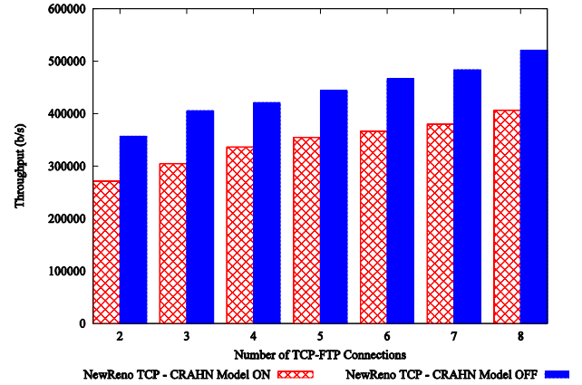
Figure 9. Multi-hop Topology: End-to-end Throughput.
