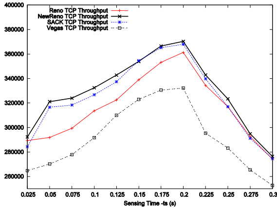
Figure 3. Sensing Cycle Analysis: TCPs Throughput.
