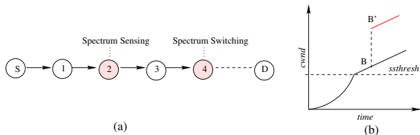
Fig. 1. A multi-hop CR ad-hoc network (a) and the forced cwnd scaling (b)
