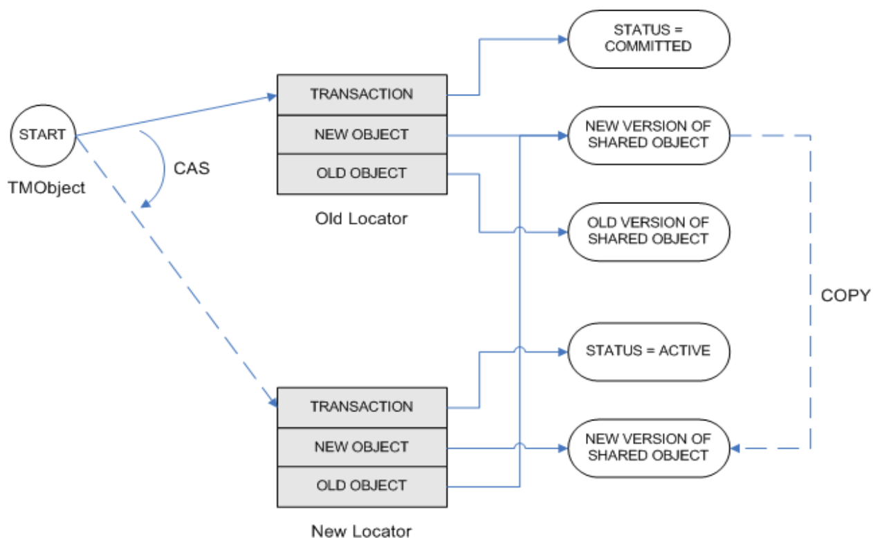
Figure 4: Opening a new transactional object (TMOBJect) in DSTM a after previous transaction commit.
